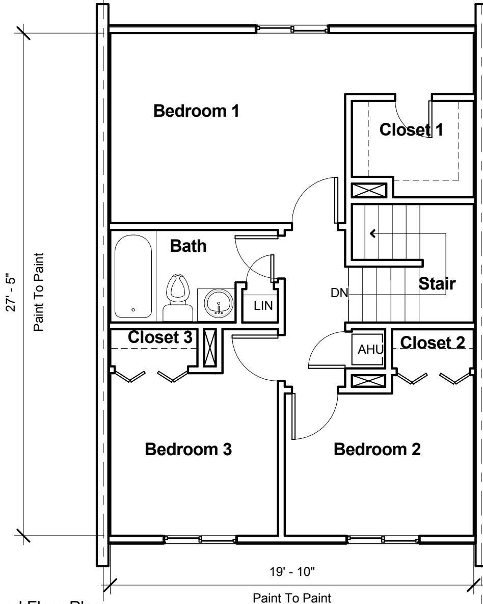
② Second Floor Plan 3/16" = 1'-0"
