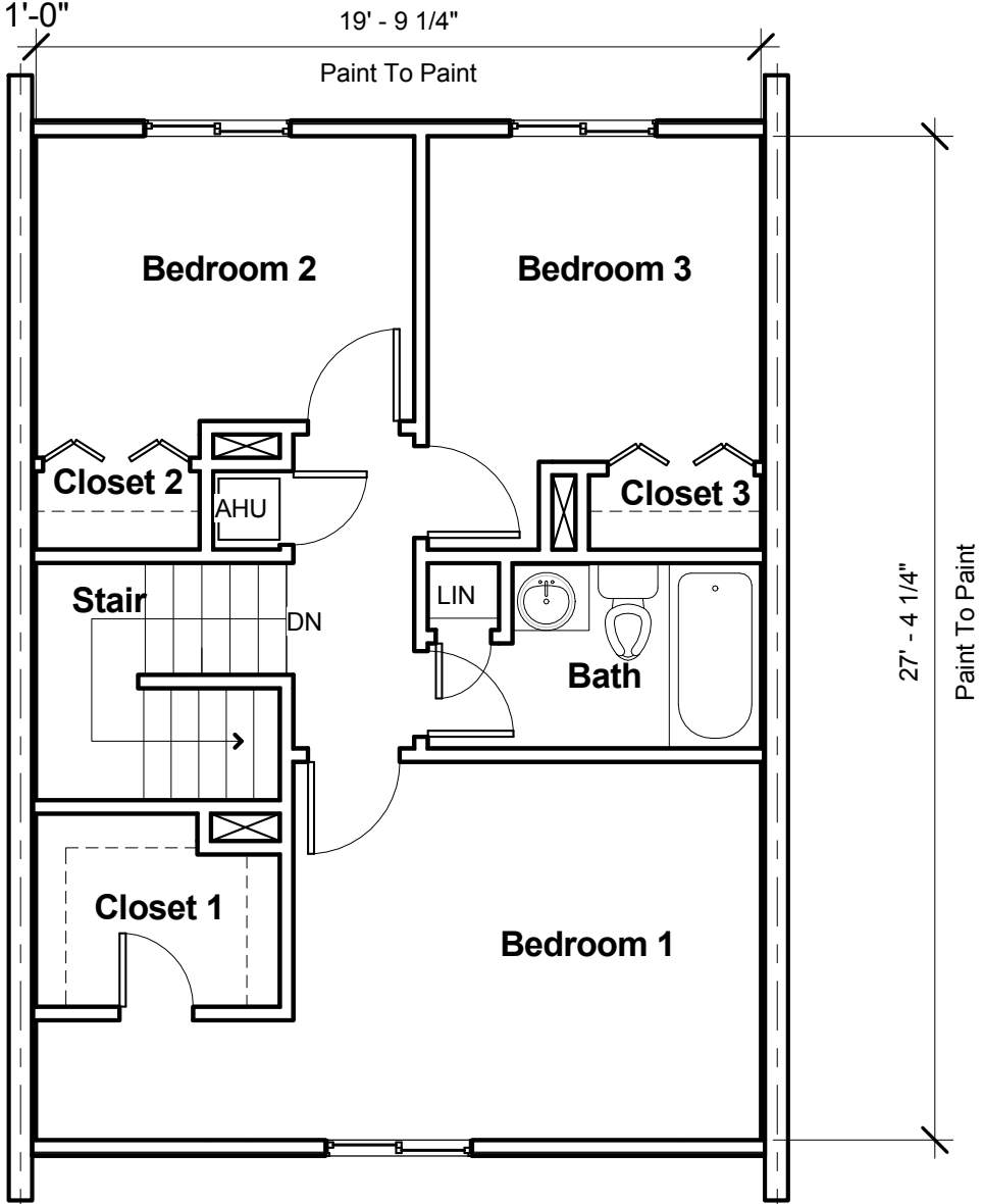
② Second Floor Plan 3/16" = 1'-0"
