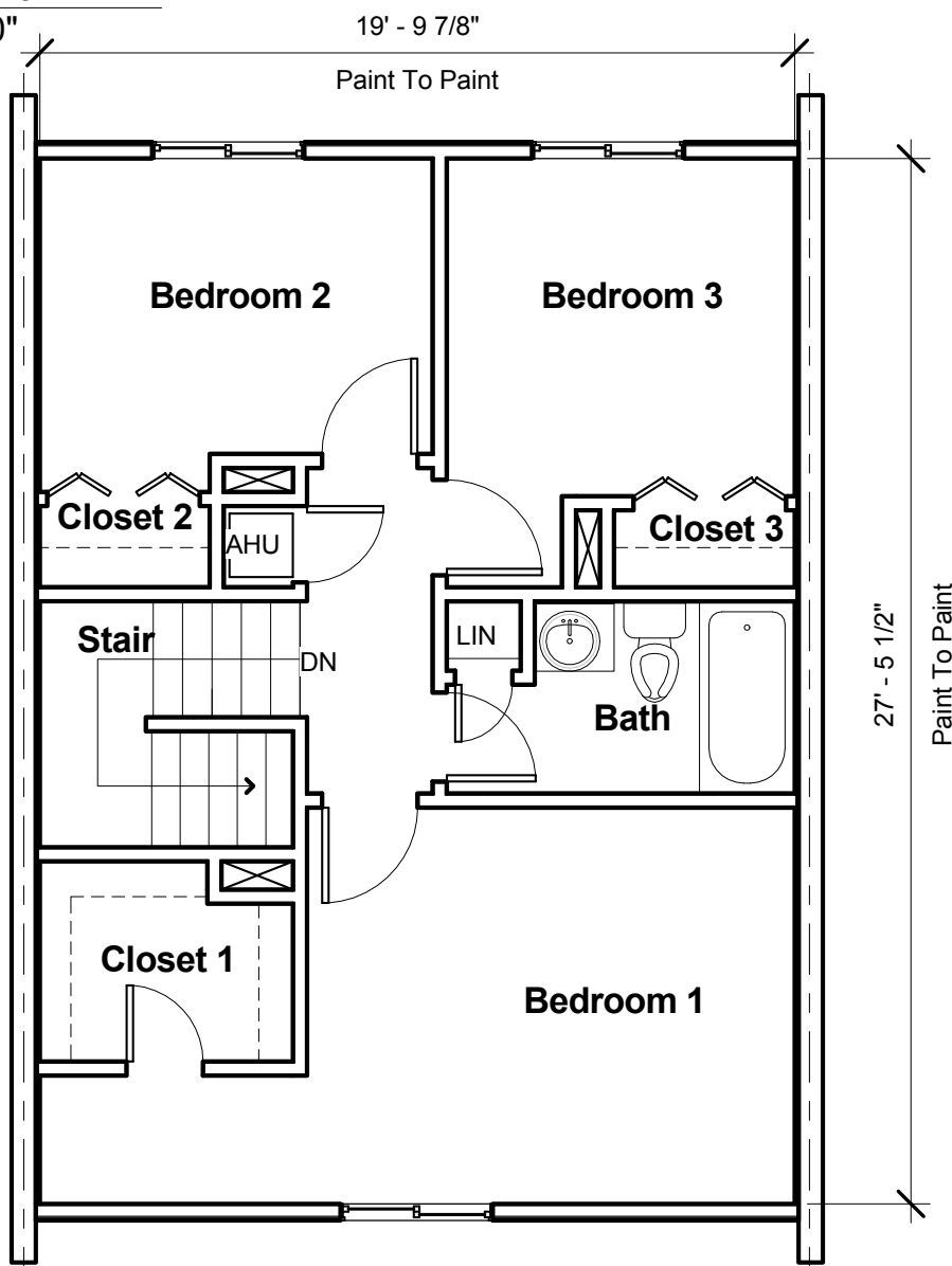
2 Second Floor Plan 3/16" = 1'-0"
