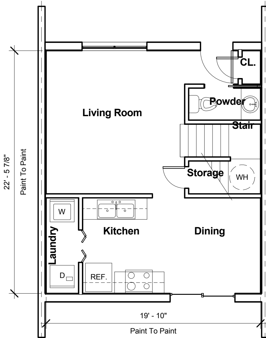
① First Floor Plan 3/16" = 1'-0"
