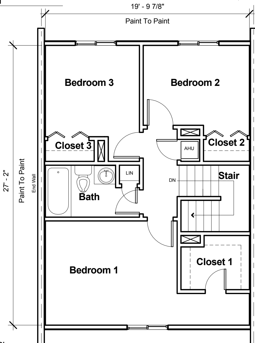
① First Floor Plan 3/16" = 1'-0"
