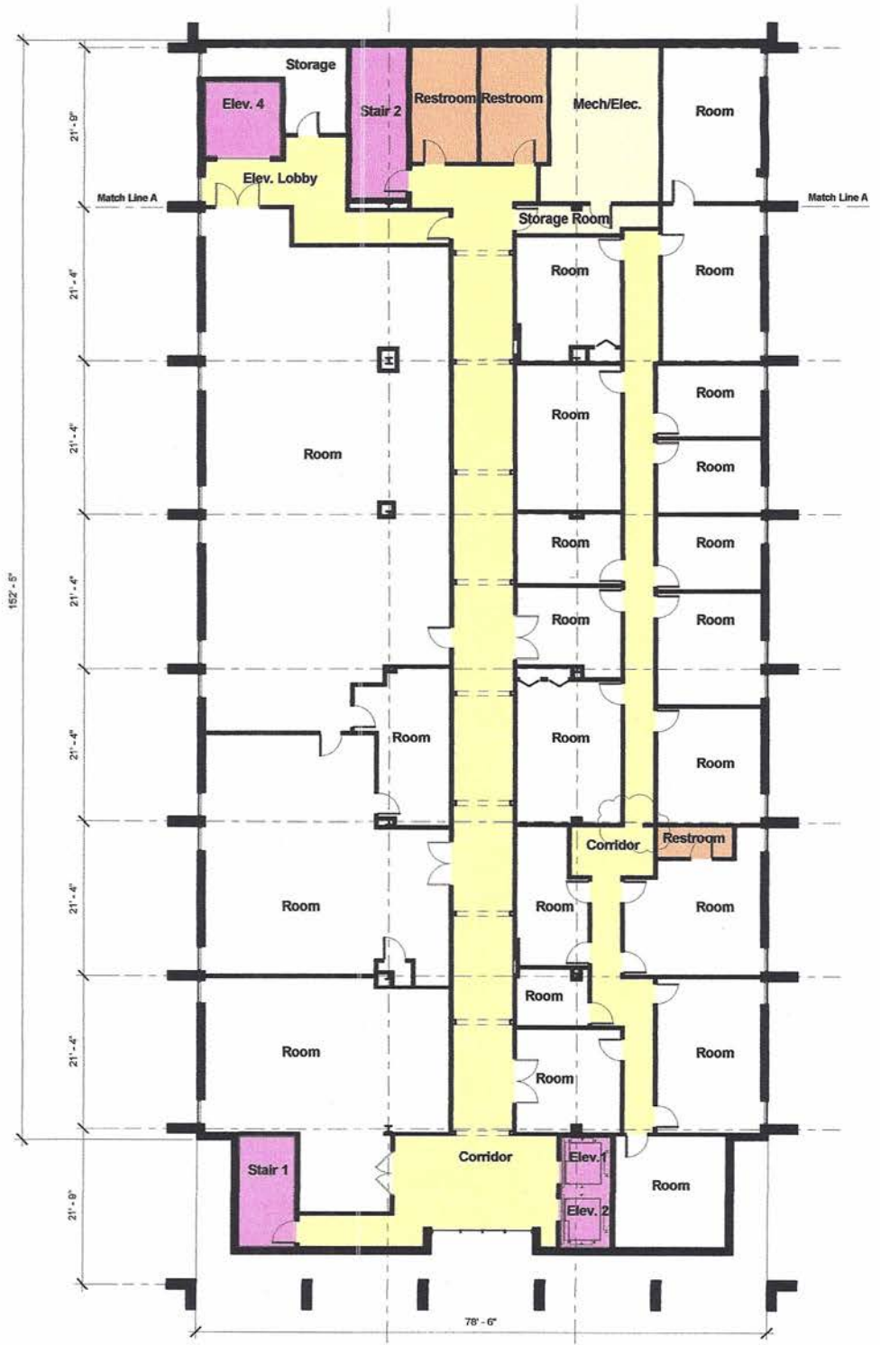
Third Floor
